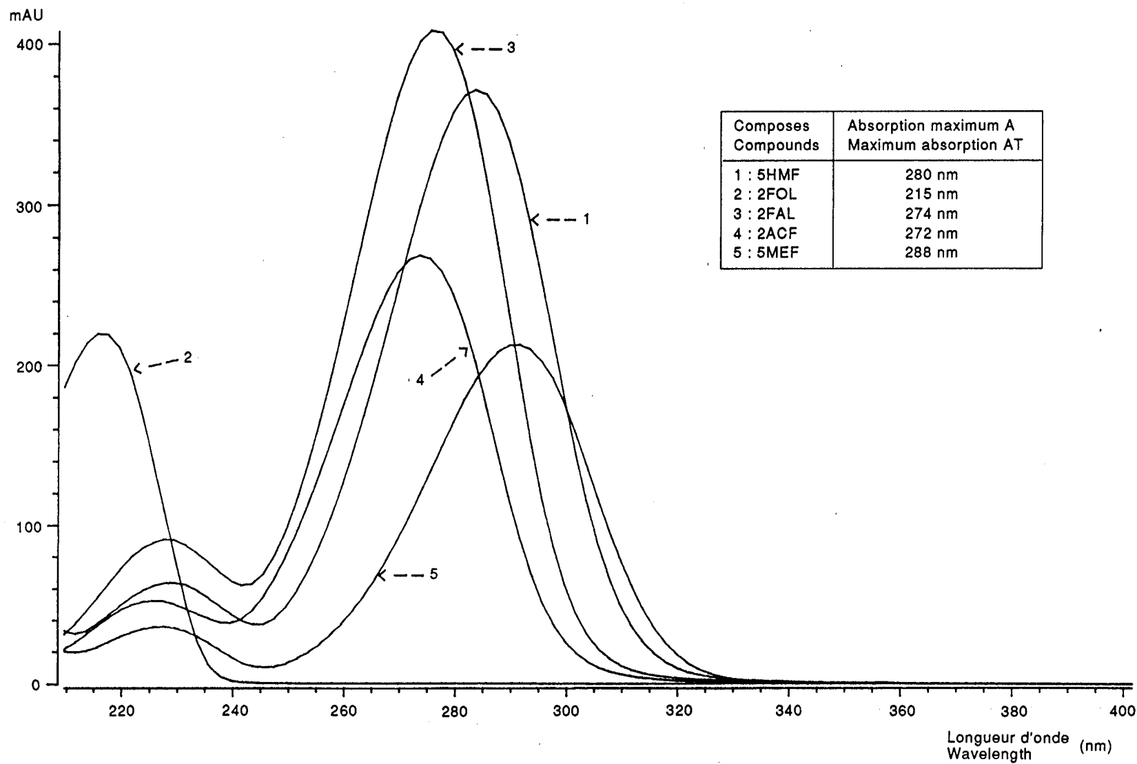
Figure 3 – Spectres UV des dérivés du 2-furfural UV spectra of the 2-furfural derivatives
